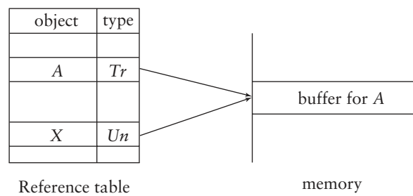
Figure 10.4: Type-Confusion Attack
